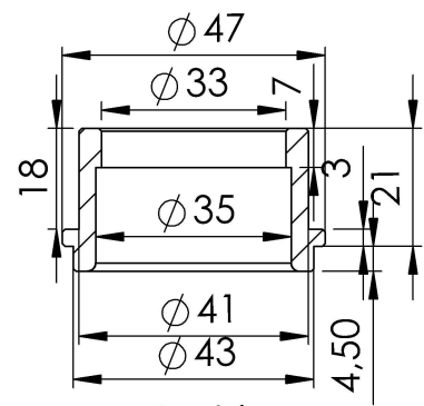
S.s. Bushing Cod.204870R
